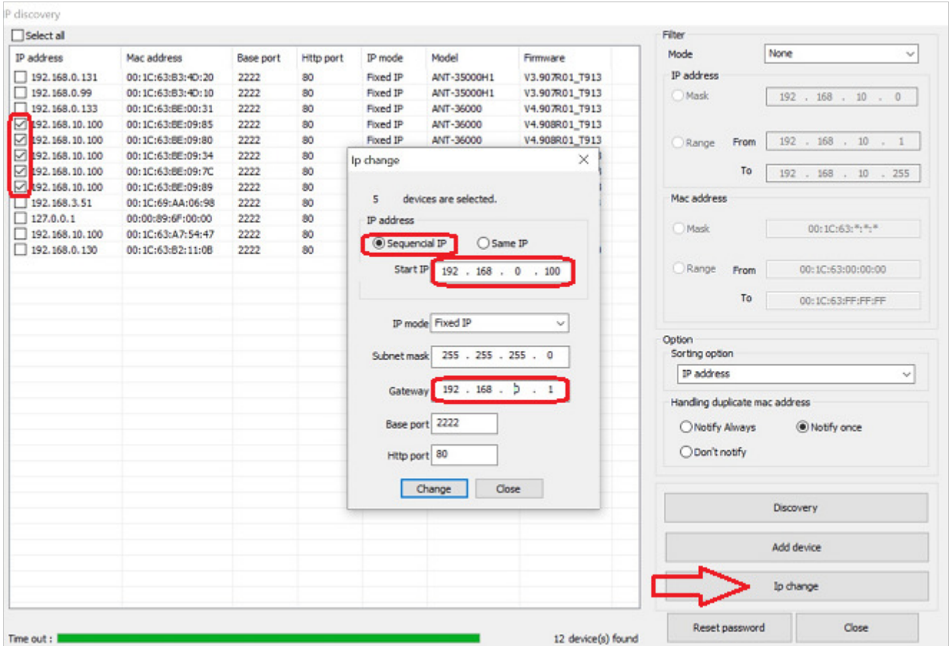
Figure 3 : select units and new IP address setting
