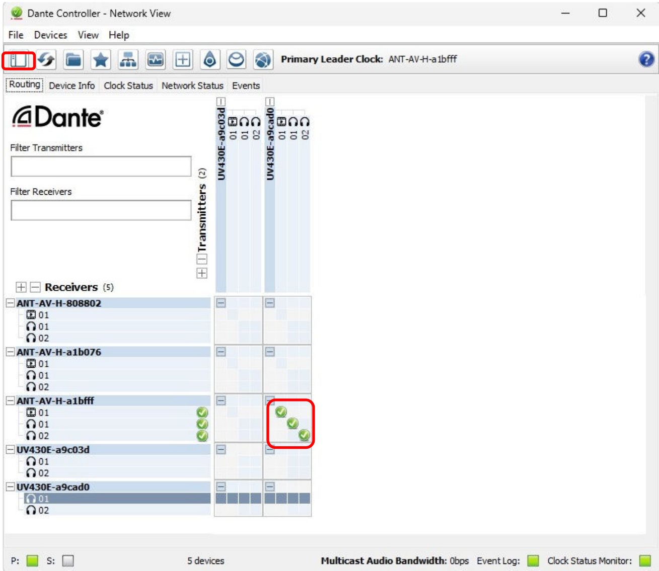
Figure 8 : Dante Controller ANT-37500 displaying video and audio
